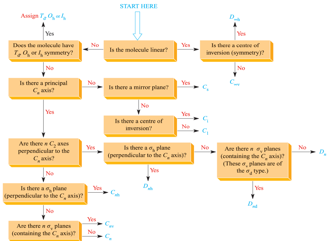
Fig. 3.10 Scheme for assigning point groups of molecules and molecular ions. Apart from the cases of n = 1 or \infty , n most commonly has values of 2, 3, 4, 5 or 6.
